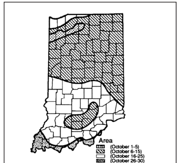
Figure 2. Average first frost dates in fall.
