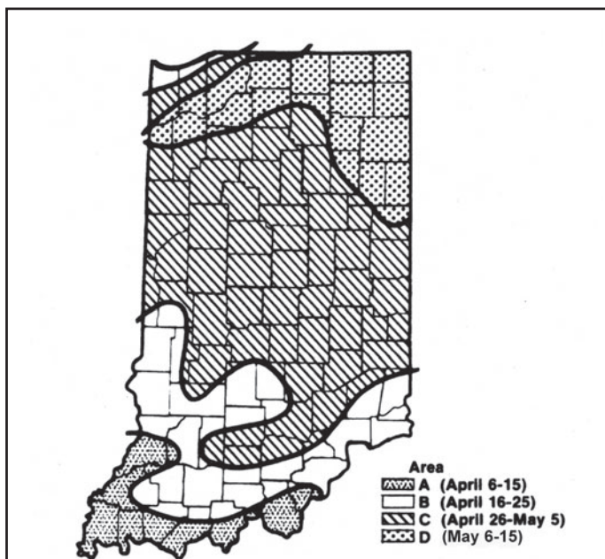
Figure 1. Average frost free dates in the spring.
