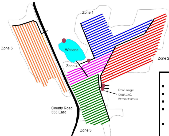
SEPEC Tile Design Plan
