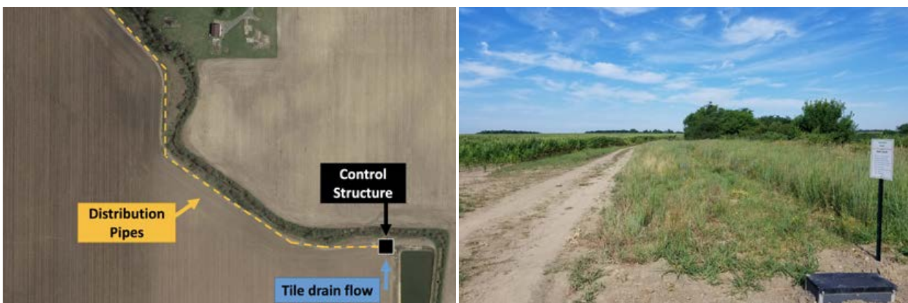
Figure F: Saturated buffer installed in Ohio along open ditch.
