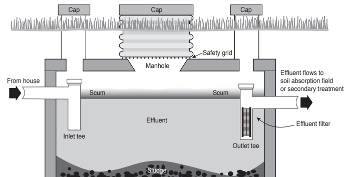
This illustration shows a cross-section of a typical septic tank.
