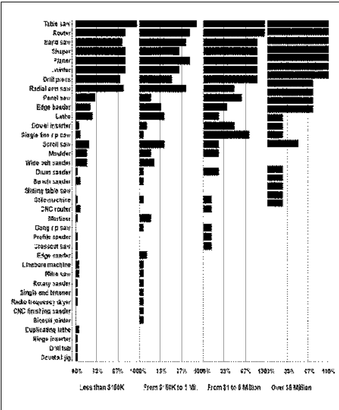
Figure 1. Average machine usage percentage in kitchen cabinet industry by machine type, by company size.
