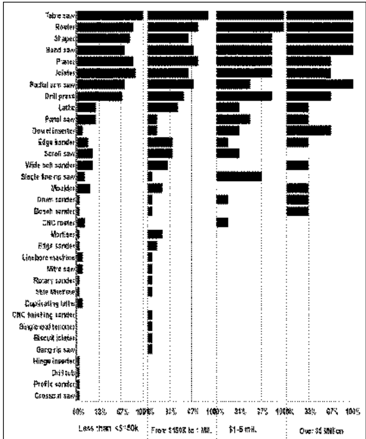
Figure 4. Average machine usage percentage in bathroom cabinet industry by machine type, by company size.
