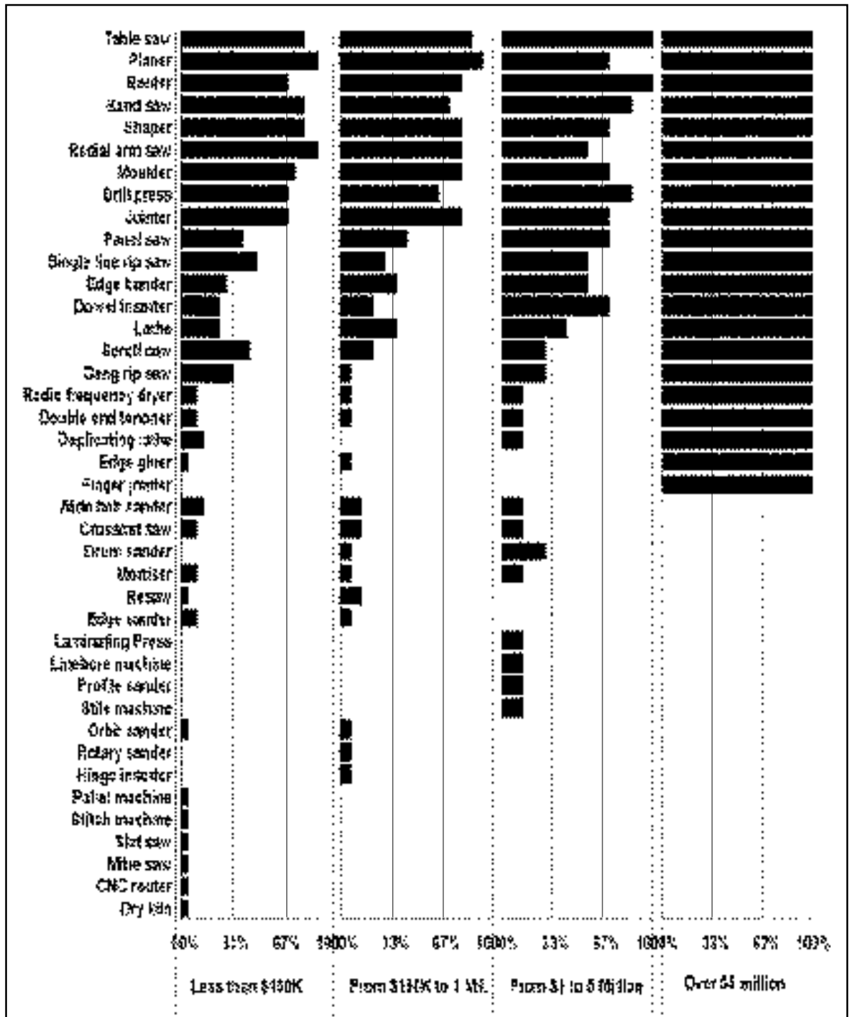
Figure 2. Average machine usage percentage in millwork industry by machine type, by company size.
